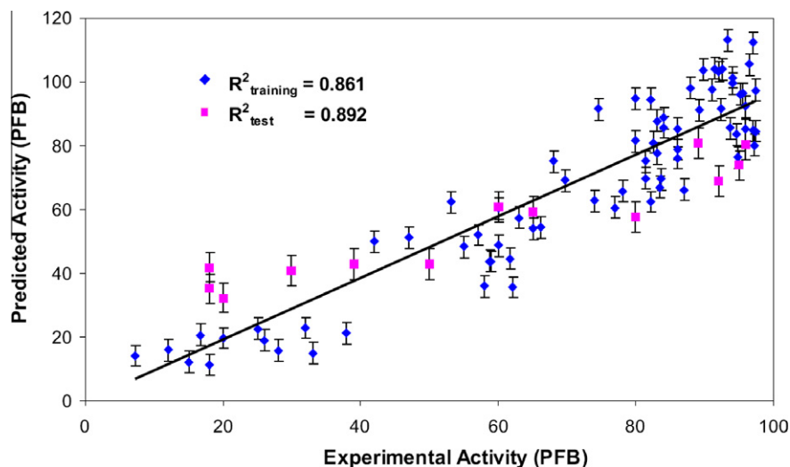
Figure 4. The plots of predicted versus experimental activities are shown by the squared correlation coefficient for training and test sets in model 1.
